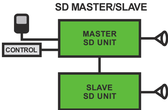
Single control/mic, multiple slaves e.g 2 x SD120=240w
