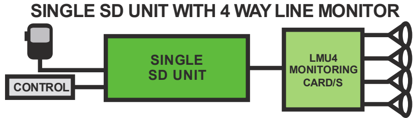
Single control/mic, multiple speaker circuits
